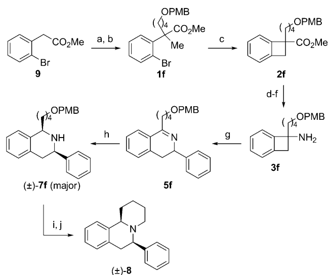
Scheme 3. Synthesis of fused heterocycle 8 . Reagents and conditions: a) NaHMDS (HMDS = hexamethyldisilazide), PMBO(CH 2 ) 4 I (PMB = p -methoxybenzyl), THF, 20 °C, 76%; b) NaHMDS, MeI, THF, 74%; c) Pd(OAc) 2 (10 mol%), P( t Bu) 3 (20 mol%), K 2 CO 3 , DMF, 140 °C, 73%; d) NaOH, MeOH/H 2 O, reflux, 85%; e) DPPA, Et 3 N, toluene, reflux, then allyl alcohol, 80 °C, 83%; f) [Pd(PPh 3 ) 4 ] (2 mol%), PPh 3 (9 mol%), 2-ethylhexanoic acid, CH 2 Cl 2 , 20 °C, 68%; g) benzaldehyde, MgSO 4 , CH 2 Cl 2 , reflux, then DMF, 160 °C, 63%; h) NaBH 4 , MeOH, 20 °C (d.r. = 7:1), 74%; i) [Ce(NH 4 ) 2 (NO 3 ) 6 ] (CAN), MeCN/H 2 O, 20 °C, 78%; j) HBF 4 , then PPh 3 , diisopropyl azodicarboxylate (DIAD), THF, reflux, 67%.
